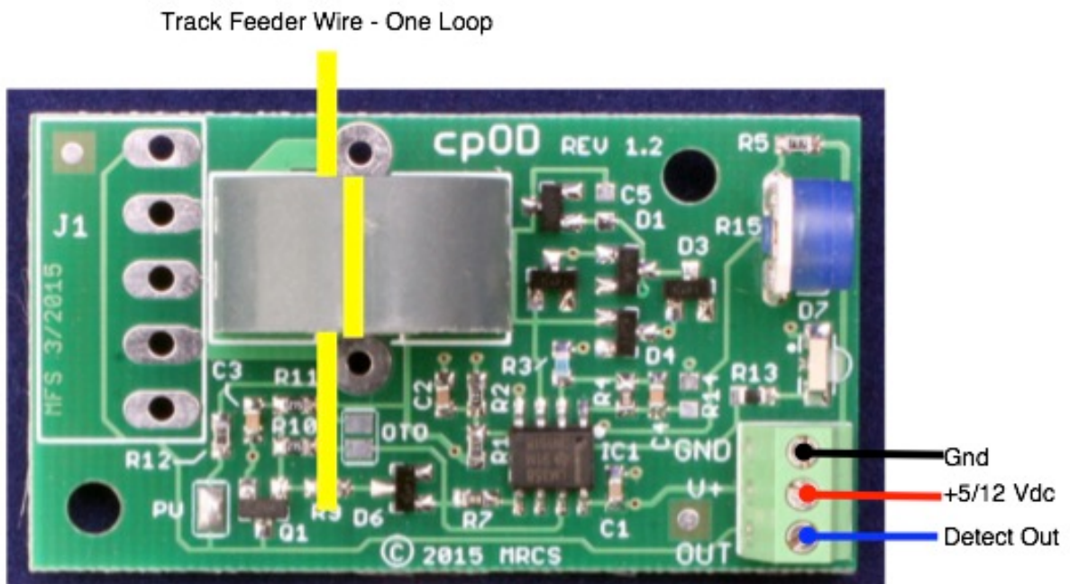
Figure 4 cpOD Connections
