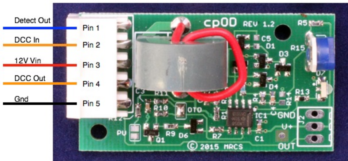
Figure 5 cpOD-M Connections
